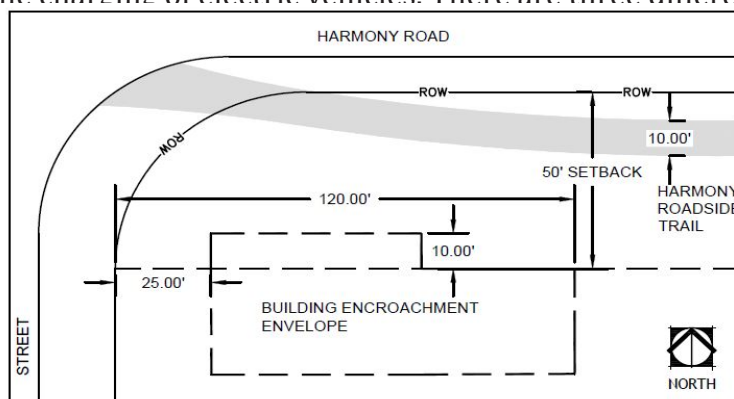
FIGURE 2 - BUILDING ENCROACHMENT INTO 50' SETBACK
